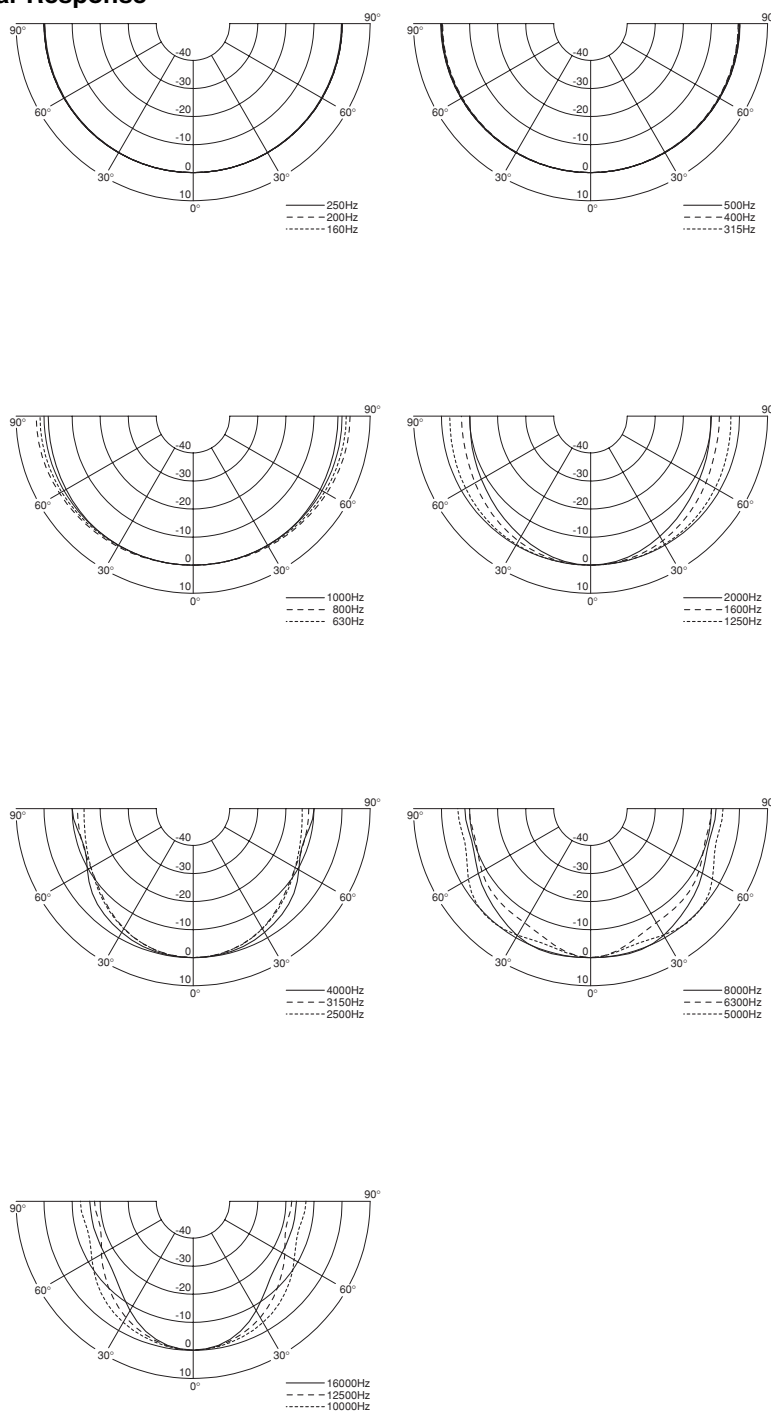
Polar Response
