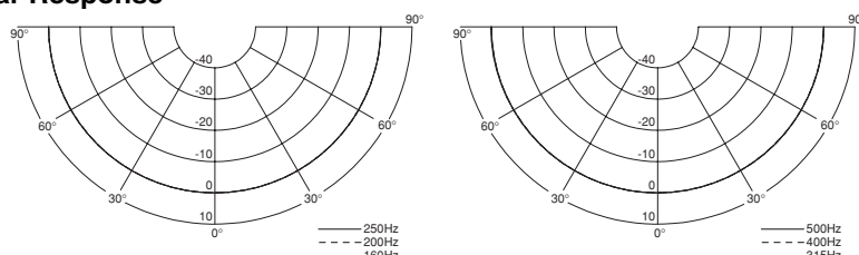
Polar Response
