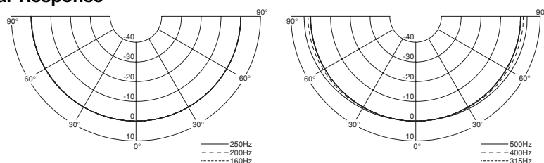
Polar Response
